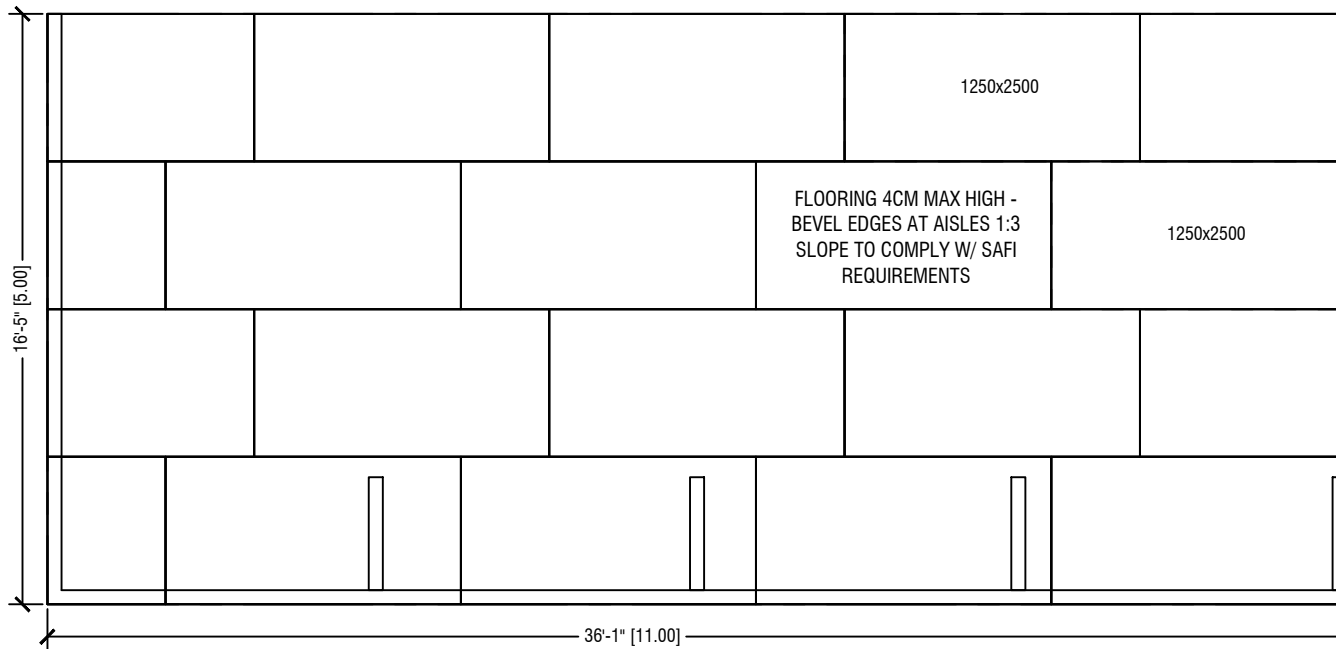
2 FLOOR FINISH PLAN
