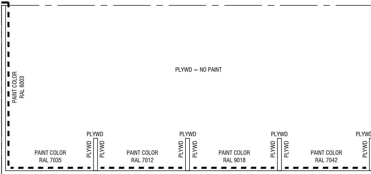
1 PAINTING PLAN
