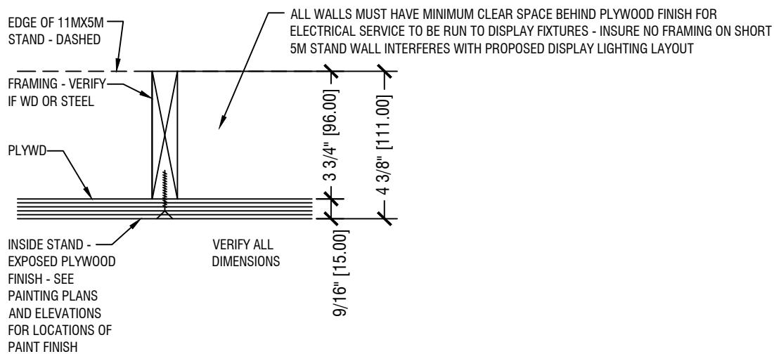
1 TYPICAL WALL AND SOFFIT CONSTRUCTION DETAIL
