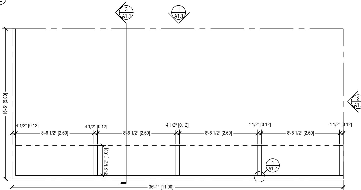
1 FLOOR PLAN
