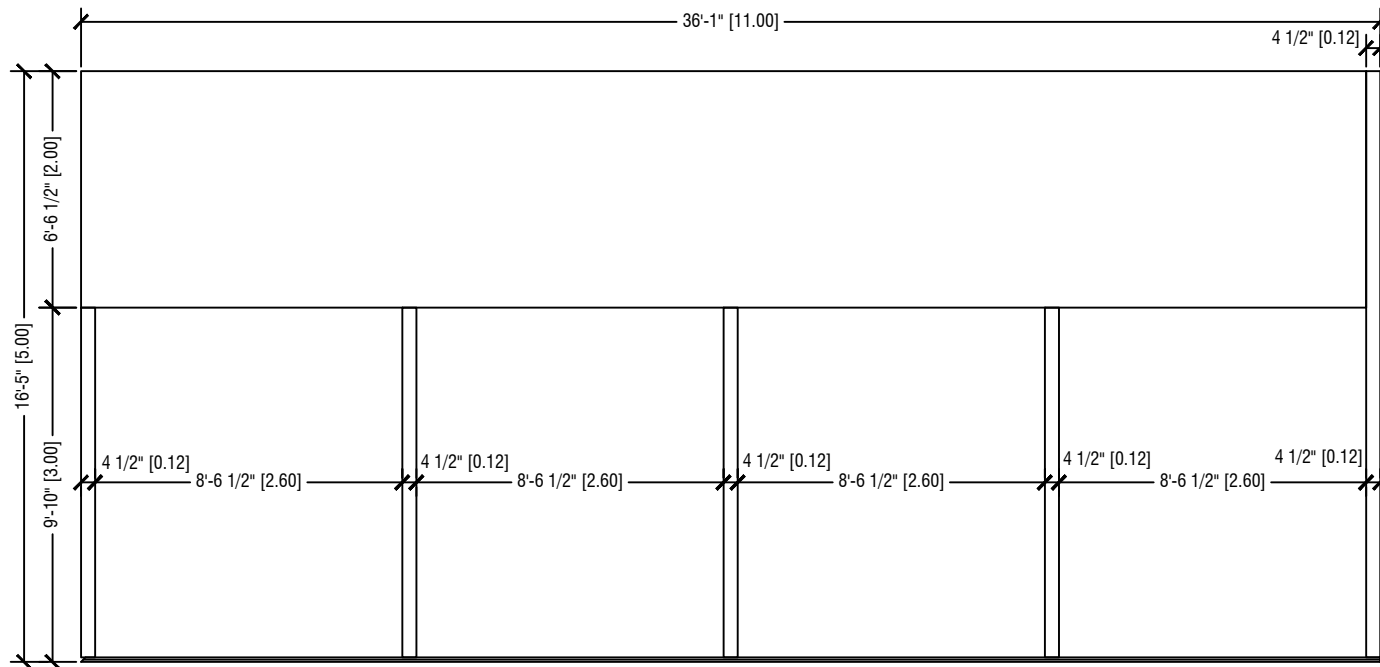
1 REAR WALL ELEVATION
