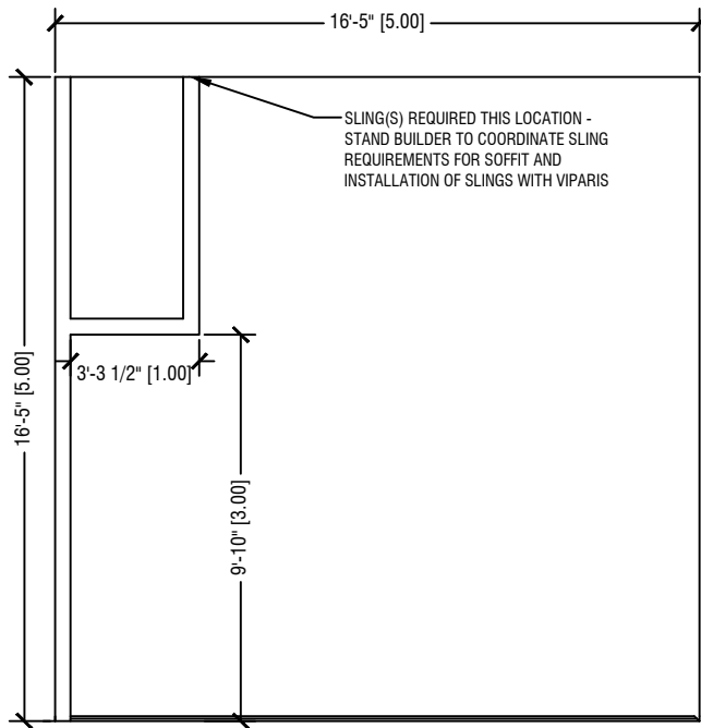
3 SECTION - SIDE WALL ELEVATION
