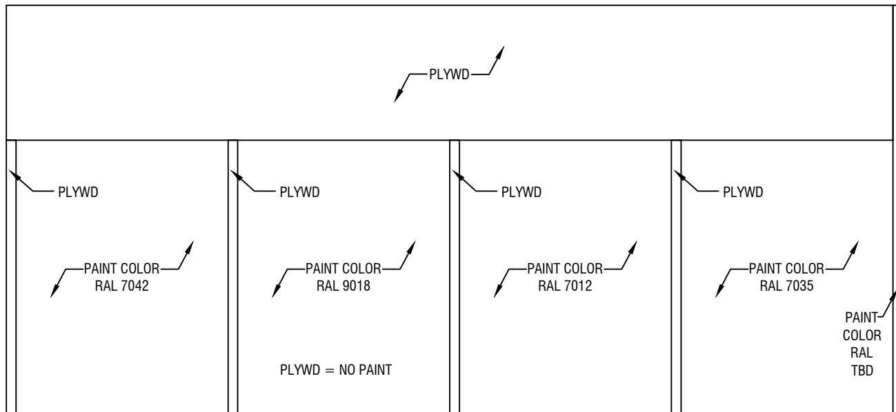
1 PAINTING REAR ELEVATION
