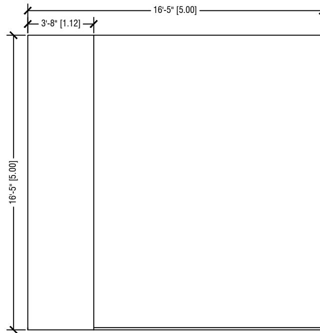
2 SIDE ELEVATION - FROM AISLE
