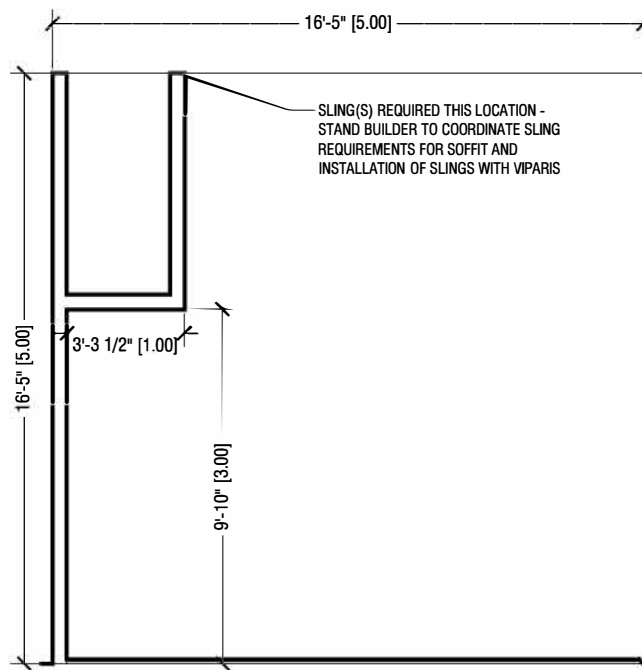
③ SECTION - SIDE WALL ELEVATION
