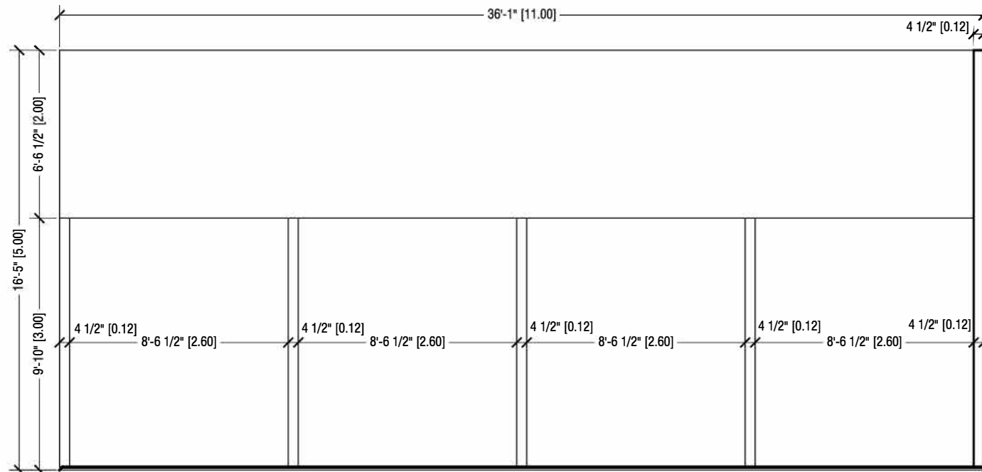
① REAR WALL ELEVATION
