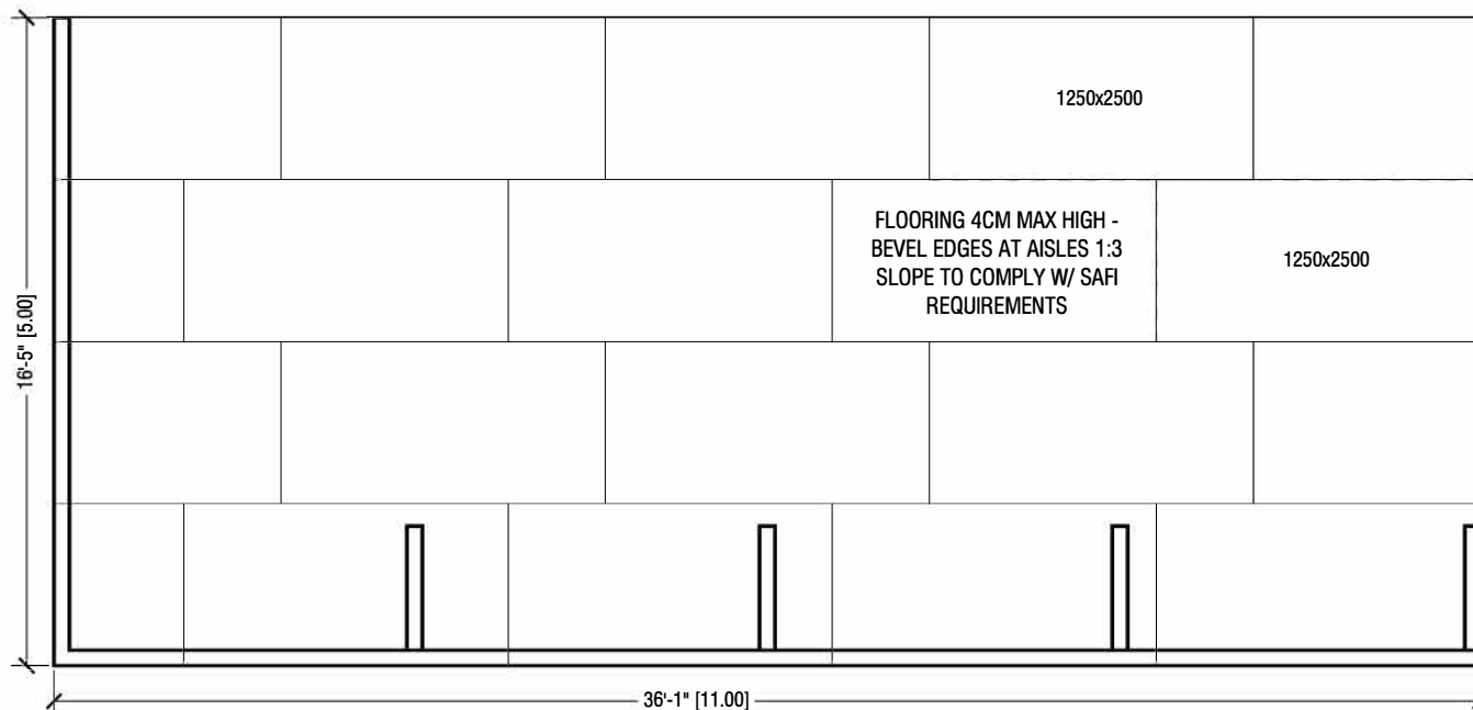
FLOOR FINISH PLAN
