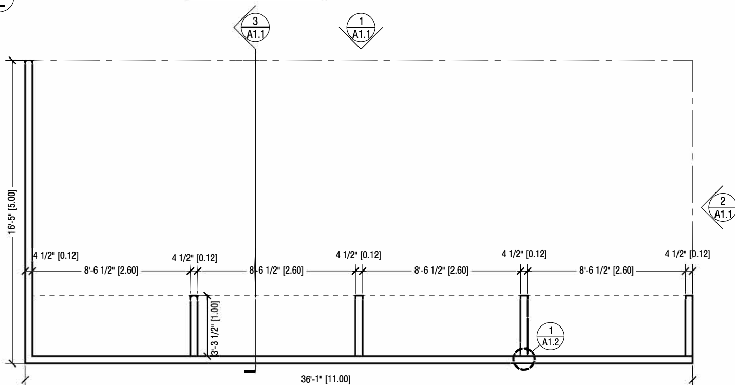
FLOOR PLAN
